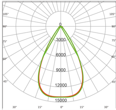
H26203 (60°) 100W Beam Angle
