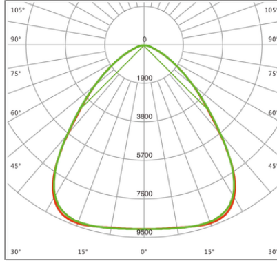
H26202 (85°) 100W Beam Angle
