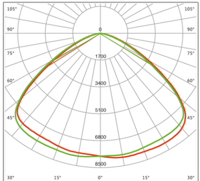
H33201 (120°) 150W Beam Angle
