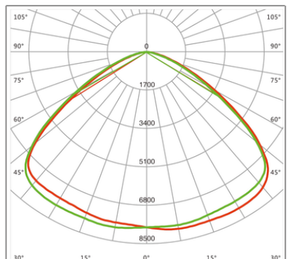
H40501 (120°) 200W Beam Angle
