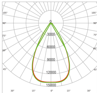
H33203 (60°) 150W Beam Angle
