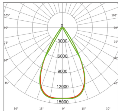
H40503 (60°) 200W Beam Angle
