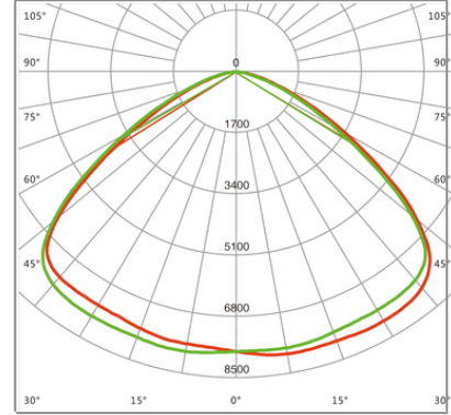
H26201 (120°) 100W Beam Angle
