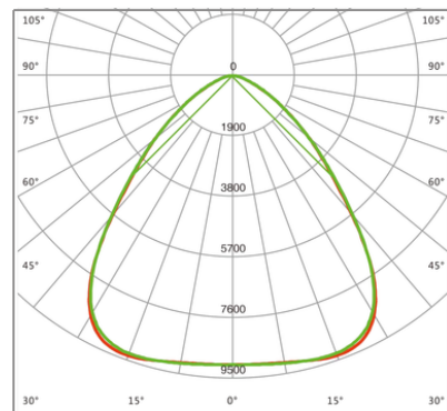
H40502 (85°) 200W Beam Angle
