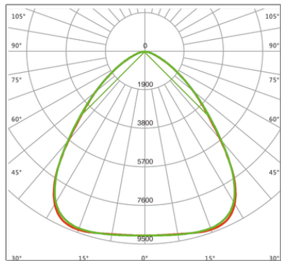
H33202 (85°) 150W Beam Angle
