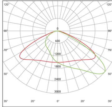
U04201 30W Beam Angle
