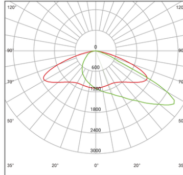
R08401 40W/70W Beam Angle
