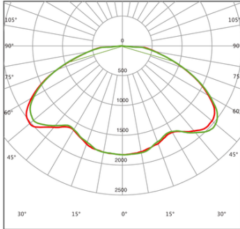
U00C09 (Type V) 25W/40W/60W Beam Angle
