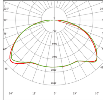
U00C07 (Type V) 80W/100W Beam Angle
